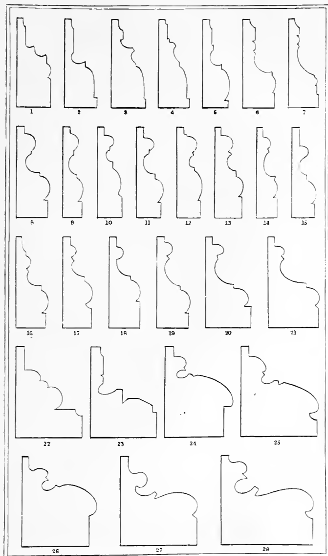
PLATE X.—PROFILES OF BASES.
